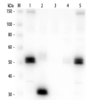
Western Blot of Anti-Rat IgG F(c) (GOAT) Antibody
