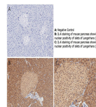
Anti-Mouse IL-6 Antibody-IHC
