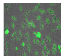
Anti-Lactate Dehydrogenase Antibody Biotin Conjugated - Immunofluorescence
