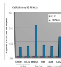
Histone H3 [Sym-dimethyl Arg8] ChIP
