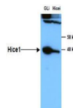
Anti-HICE1 Antibody - Western Blot
