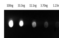
Dot Blot of Anti-Guinea Pig IgG Antibody Fluorescein Conjugate
