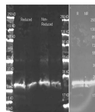
Anti GST Polyclonal Antibody-Western blot
