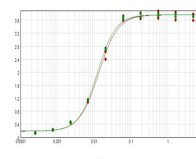
ELISA results of purified Rabbit Anti-Goat IgG F(ab') 2 Antibody
