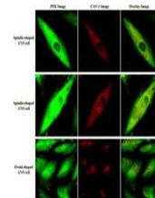
anti-F6PK MAGP-2 Antibody - Immunofluorescence Microscopy
