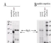
Anti-Fbp5B Antibody - Western Blot
