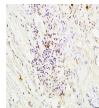
IHC-P of GRP490
