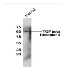
WB of GRP376
