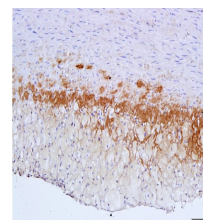
IHC-P of GRP376
