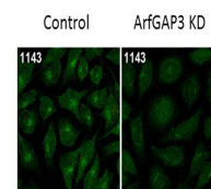
Immunofluorescence Microscopy - Anti-ArfGAP3 Antibody
