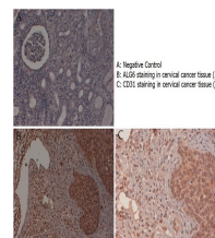
Immunohistochemistry of ALG6 Antibody
