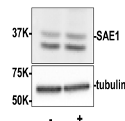
Western Blot - SAE1 Antibody
