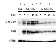
Western Blot - STAT2pS734
